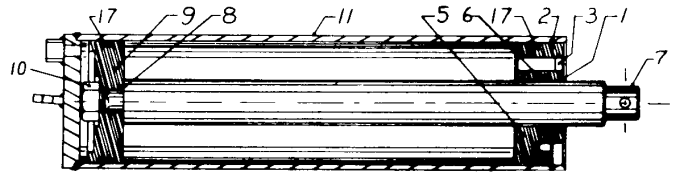
LP SERIES 6" CYLINDER
