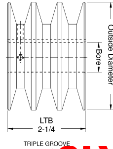
TRIPLE GROOVE
