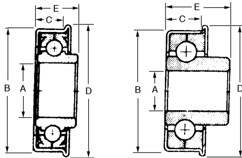
Type F Shielded Type SF Shielded & Sealed Type 150 Shielded
