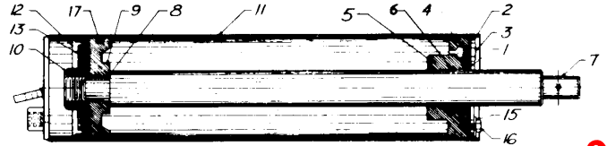
LP SERIES 5" CYLINDER
