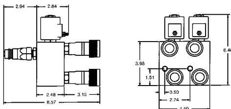
Two circuit shown with couplers
